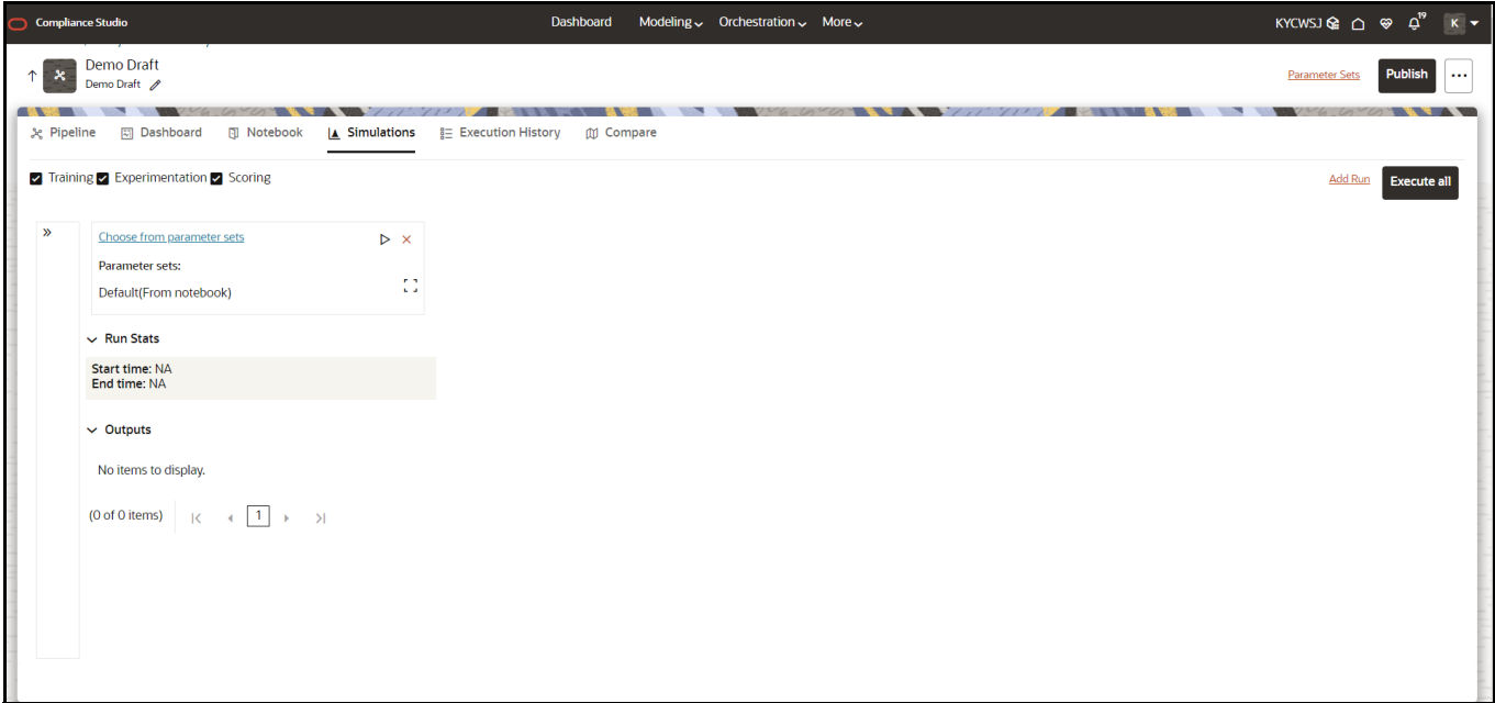
Figure 96: Simulations
