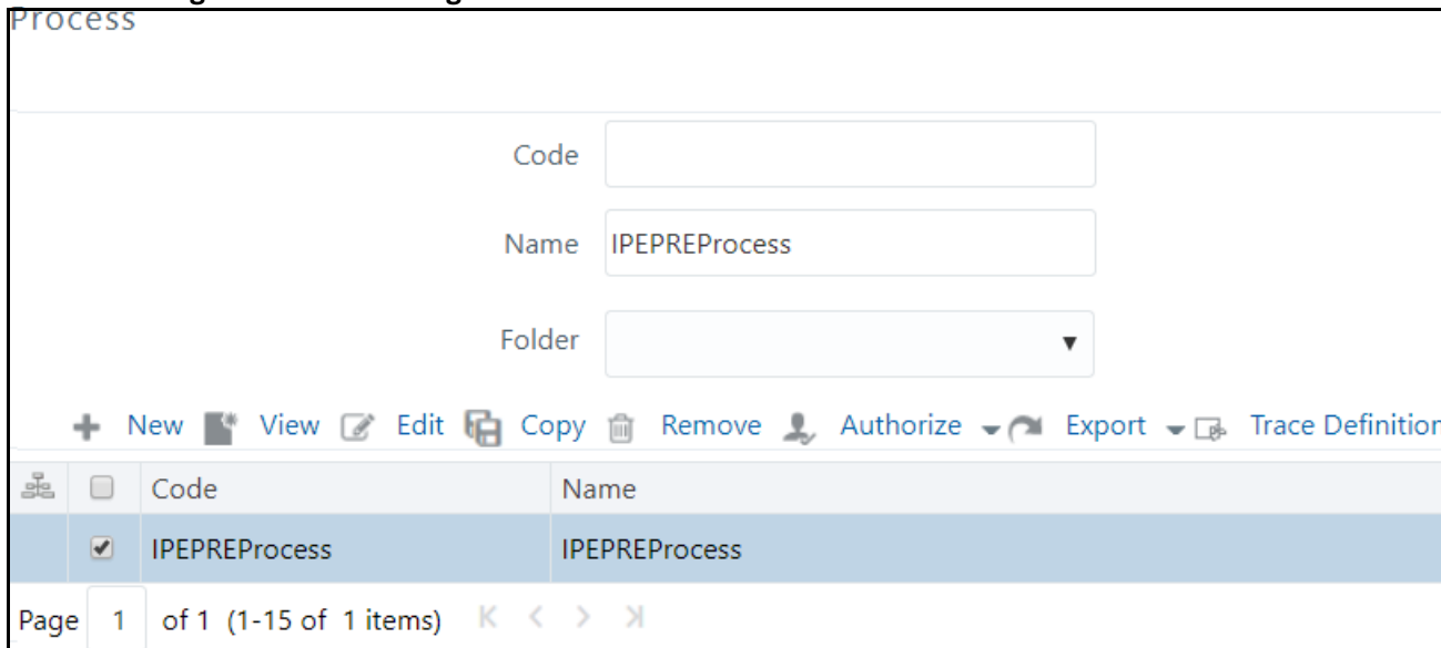
Figure 112: Process Page
