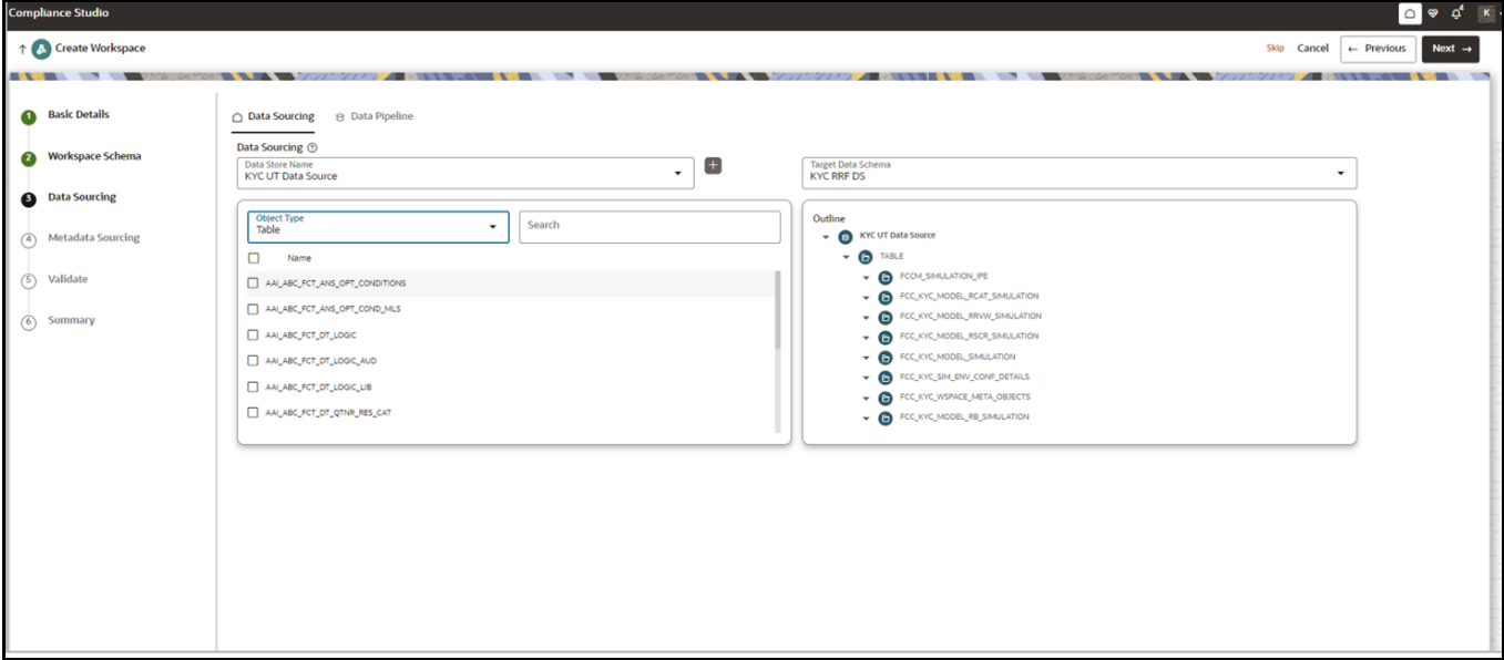
Figure 85: Data Sourcing
