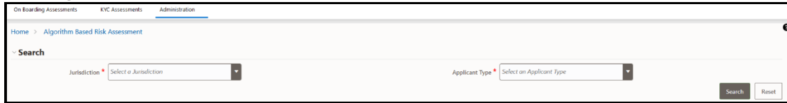
Figure 28: Search Fields
