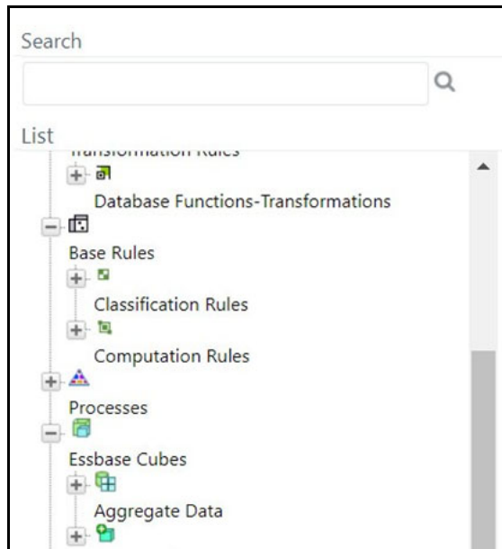
Figure 114: Component Selector
