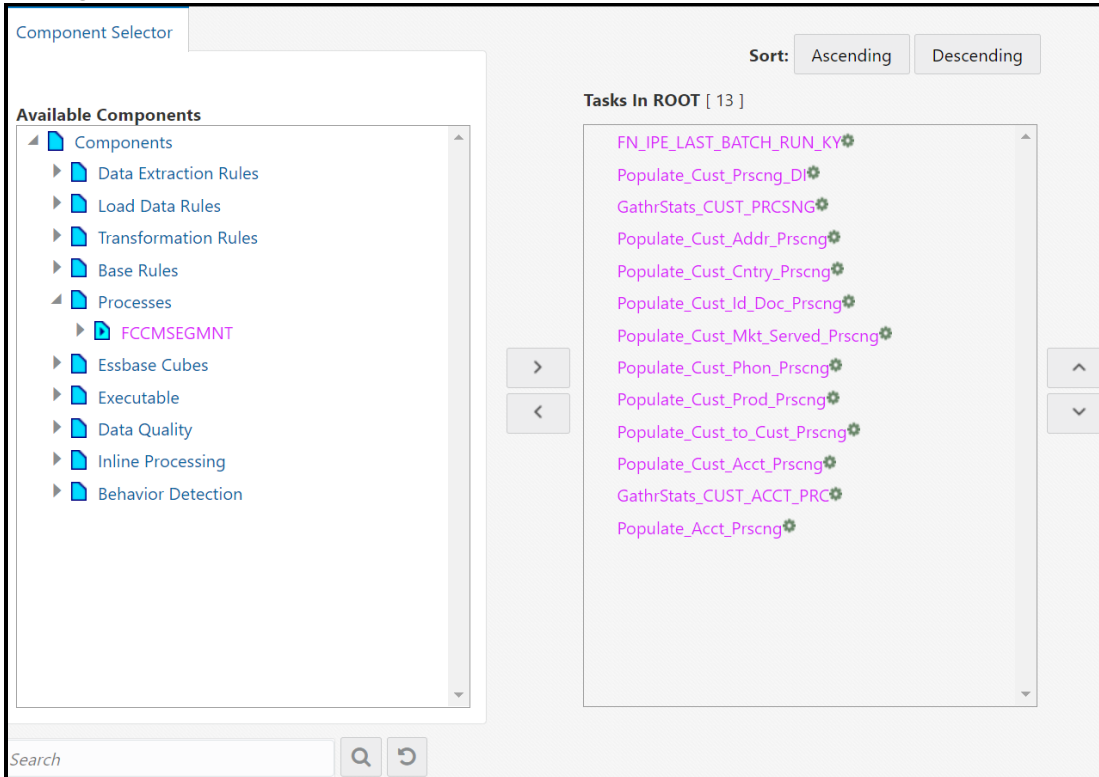
Figure 119: Component Selector
