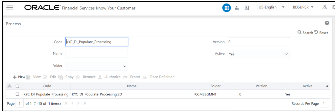
Figure 117: Process Page
