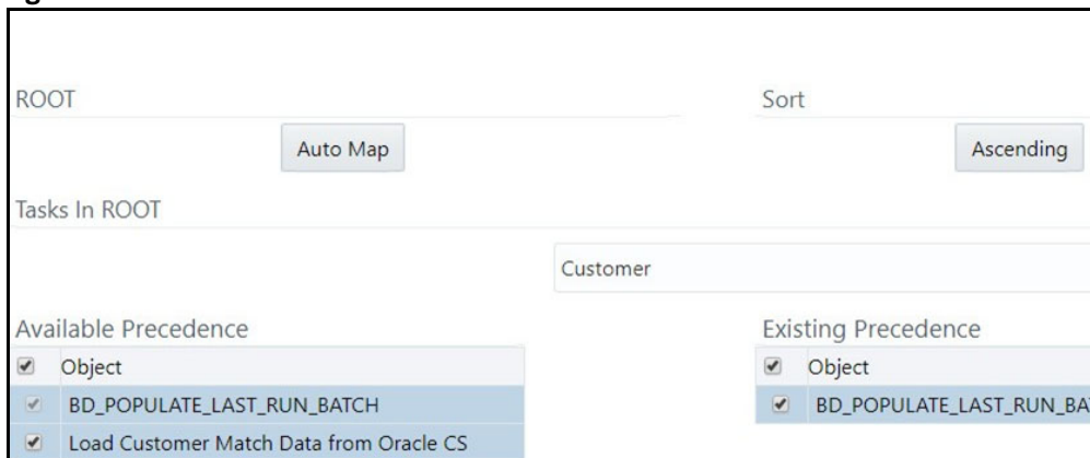
Figure 116: Precedence Selector
